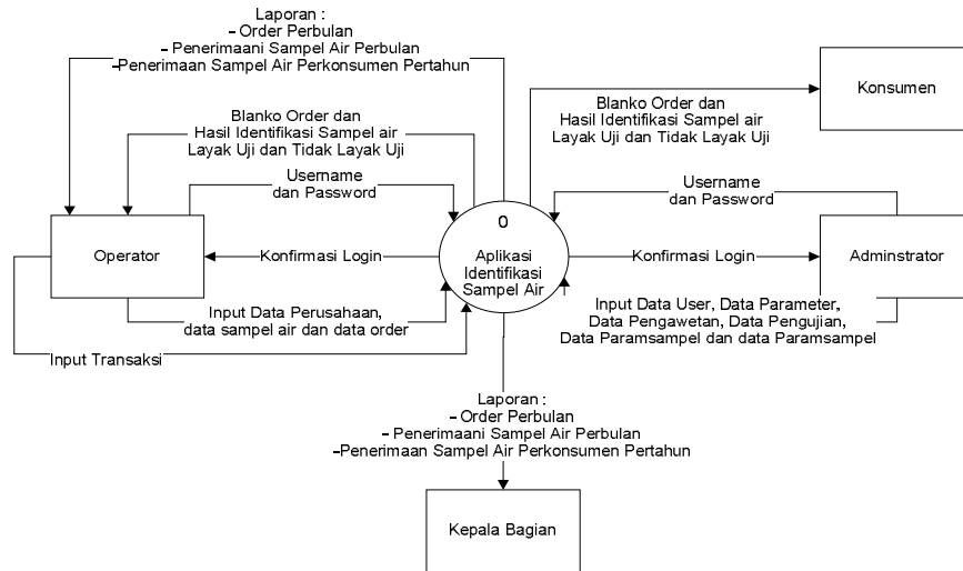
Gambar 1. Context Diagram
