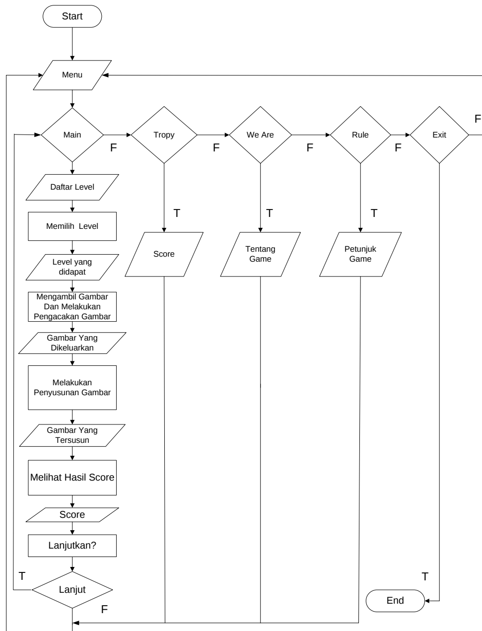
Gambar 2. Flowchart Sistem
