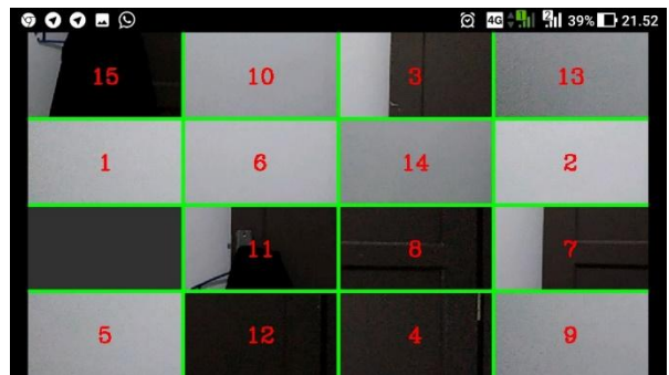
Gambar 10. Level Hard
