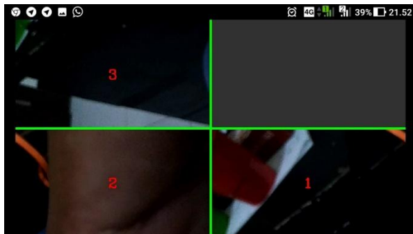
Gambar 8. Level Easy
