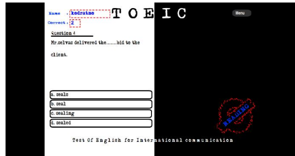
Gambar 5. Tampilan reading
